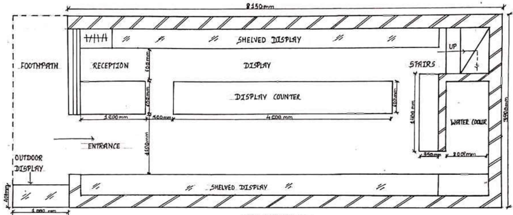
PLAN 7700x3000mm
